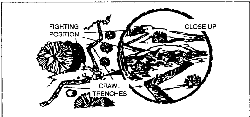
Figure 2-56. Trenches.
